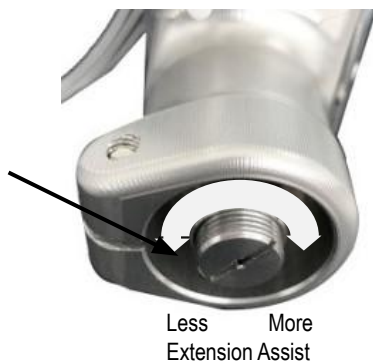
Fig. 3 Note that the screw is inside the tube clamp. (Screw accessed by removing pylon from knee unit tube clamp)
