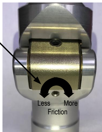
Fig. 2 Clockwise = increased friction Anti-Clockwise = reduced friction
